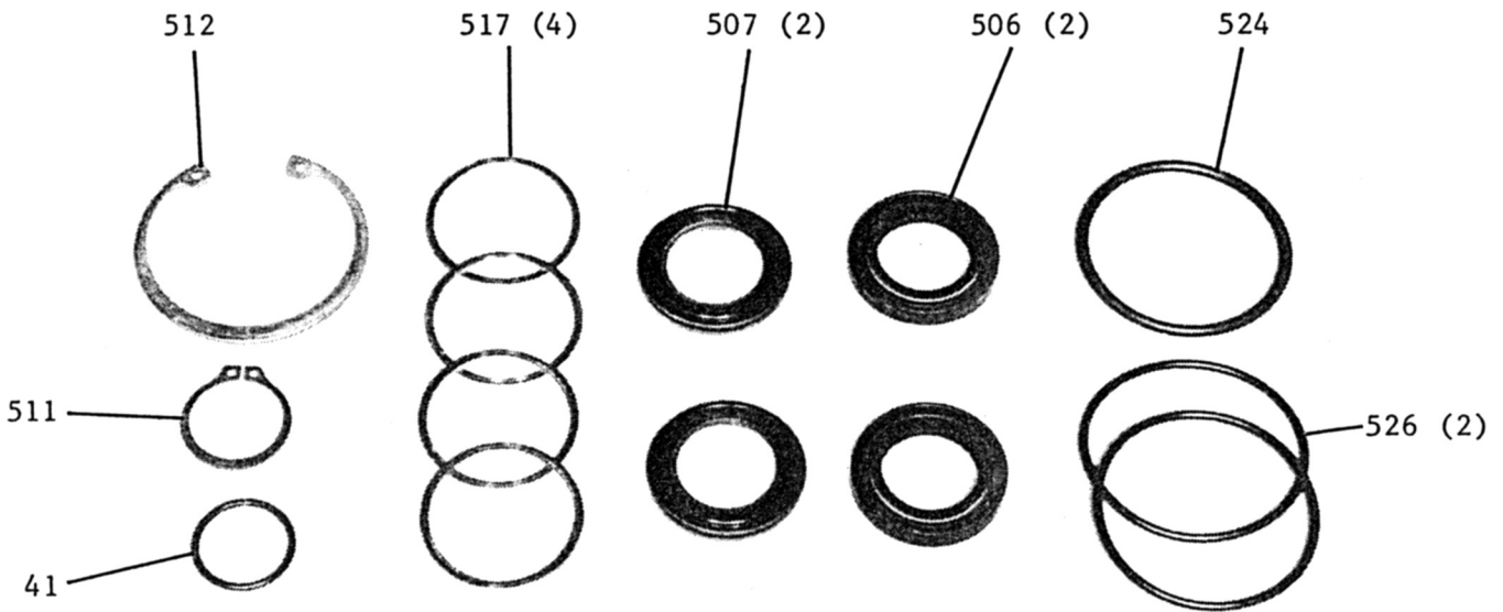
SEAL, SNAP & "O" RING KIT 803
