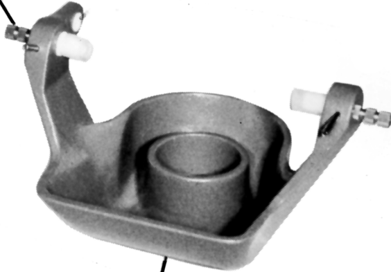
REVERSE GATE Pivot bushings in main hsg See Table Below
